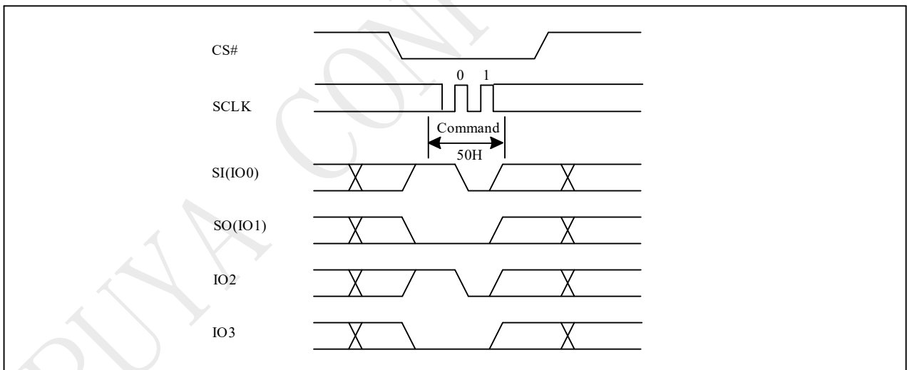
Figure 9-4a Write Enable for Volatile Register Sequence (QPI)
