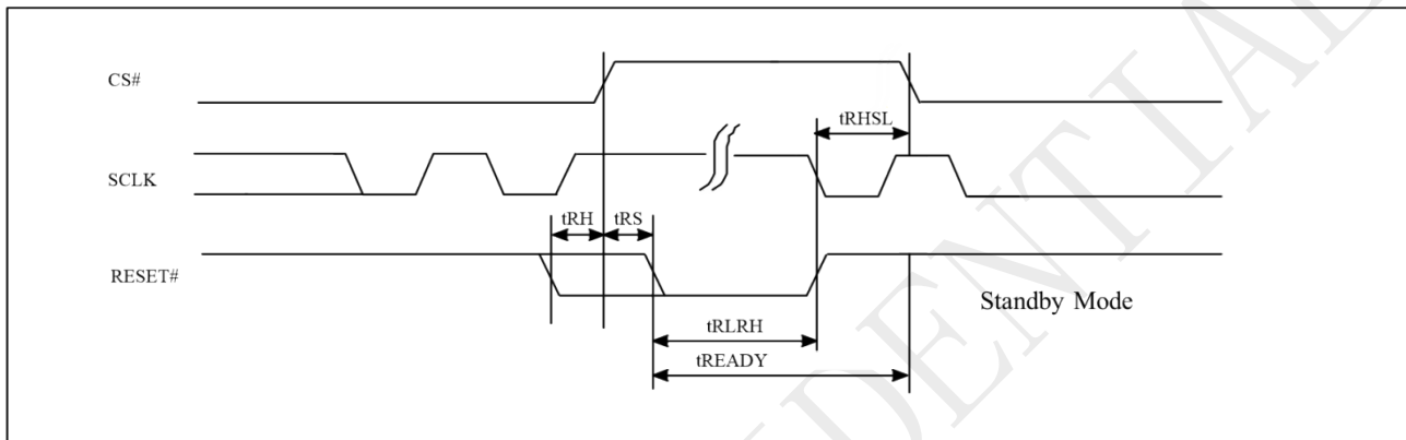
Figure 9-51 RESET Timing
