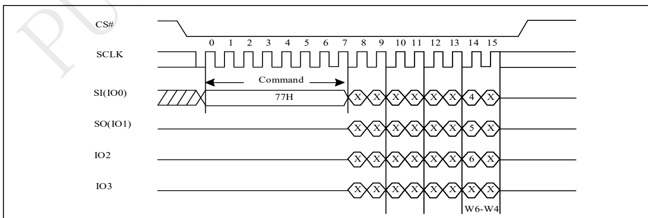
Figure 9-17 Set Burst Read (SBL) Sequence (Command 77h)
