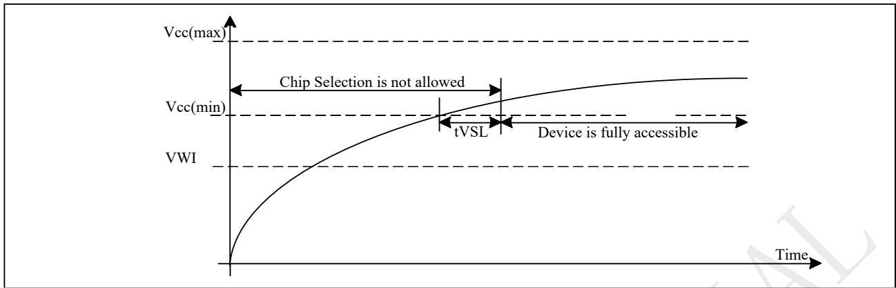
Figure 5-7 Power-Up Timing
