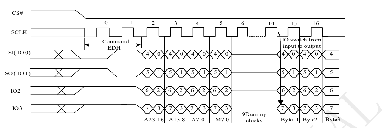
Figure 9-18b DTR 4IO Read Mode Sequence (QPI EDh M5-4 ≠ (1,0))
