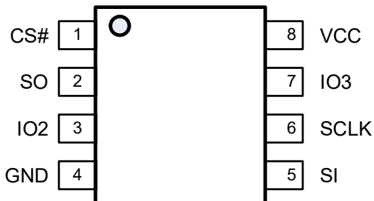
Figure 3-1 for SOP8 package
